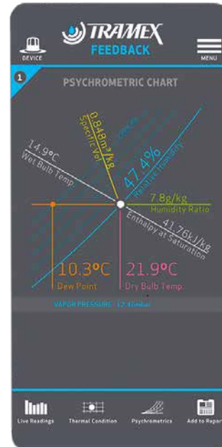
Psychrometric Chart
